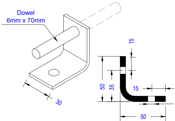
3mm Stainless steel cramp fixing
