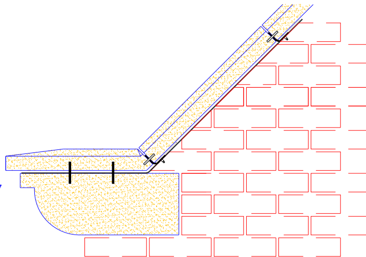
3mm Stainless steel cramp fixing
