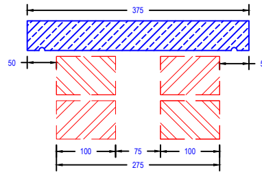
Coping Section to CP3
