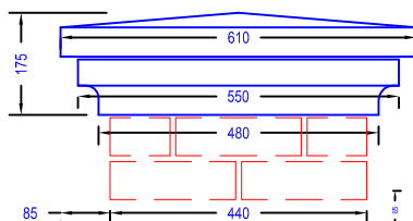
Capping PC3 610 x 610 x 75 with MB3 = 550 x 550 x 75
