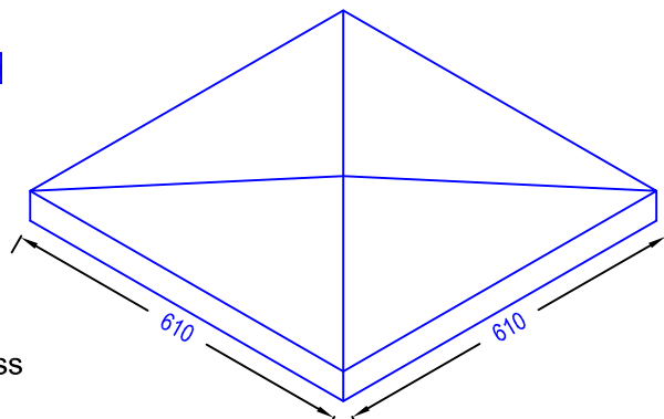
Capping PC3 610 x 610 x 75
