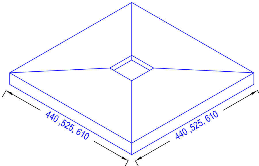
Sphere Base SB1= 440, SB2 = 525. SB3= 610,
