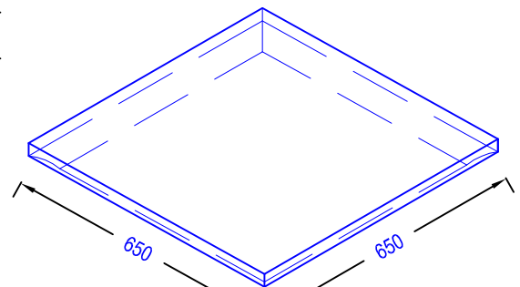
Sub Base to Capping MB2
