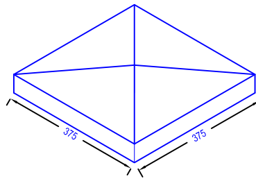
Capping P2 375 x 375 x 75
