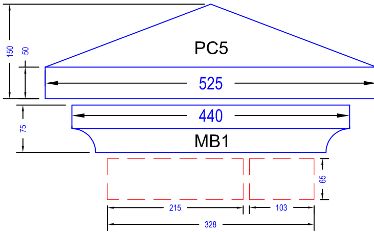
Capping PC5 with MB1
