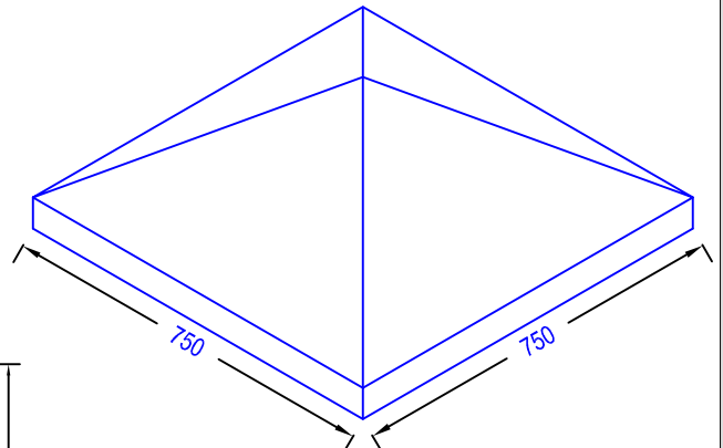
Capping PC4 750 x 750 x 200
