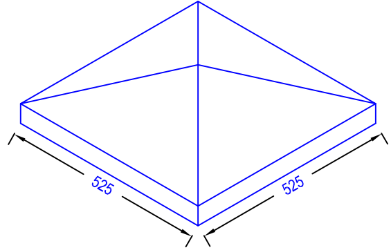
Capping PC5 525 x 525 x 150
