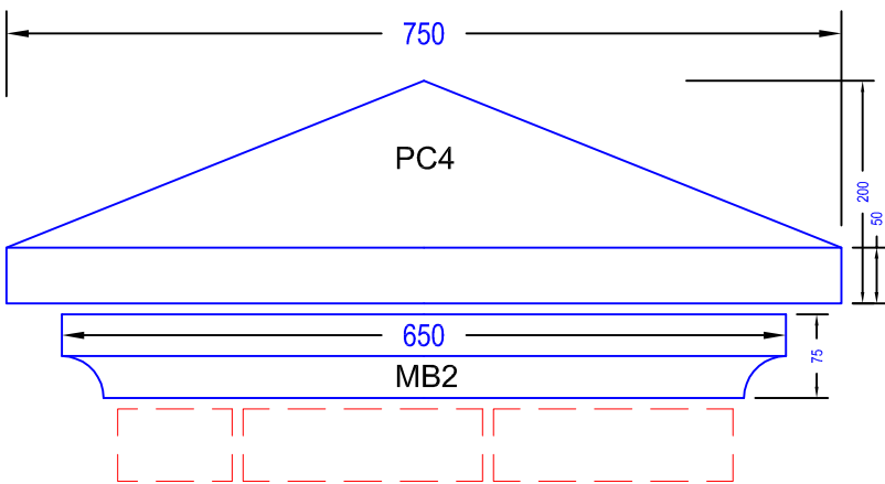
Capping PC4 with MB2
