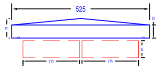
Capping PC2 = 525 x 525 x 75
