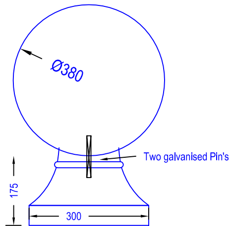
Finial Base SF3/380
