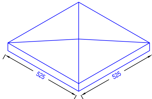
Capping PC2 525 x 525 x 75
