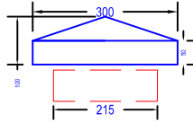
Capping P1 = 300 x 300 x 100
