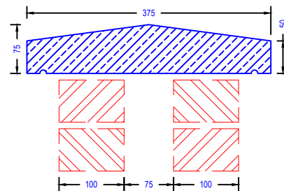
Coping Section CP4/375
