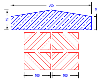
Coping Section CP4/305
