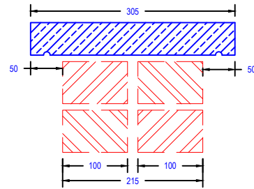
Coping Section to CP2
